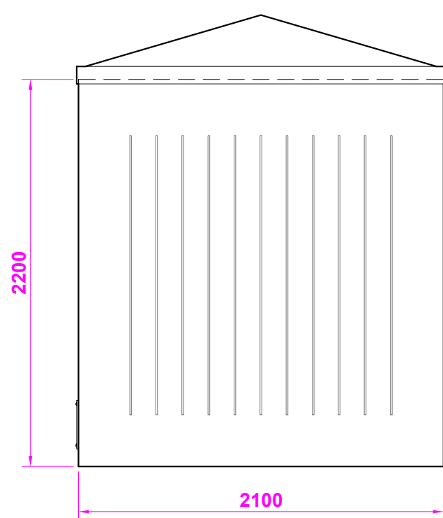
Elevation (C) (rear)
