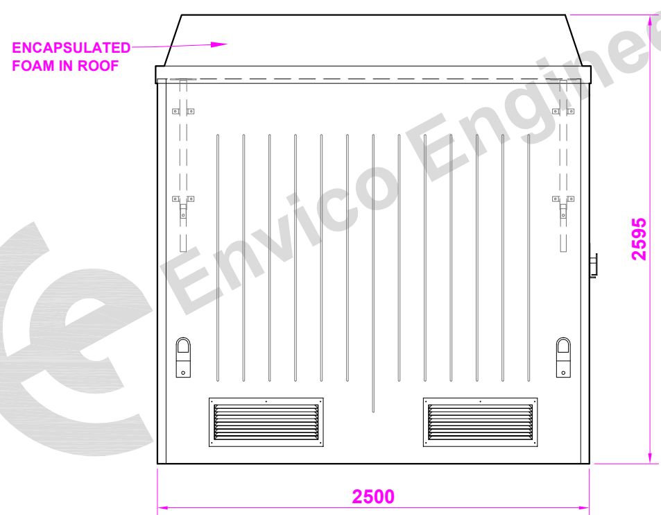
Elevation (B) (l/h side)
