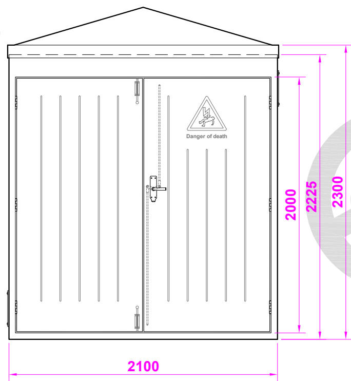
Elevation (A) (front)
