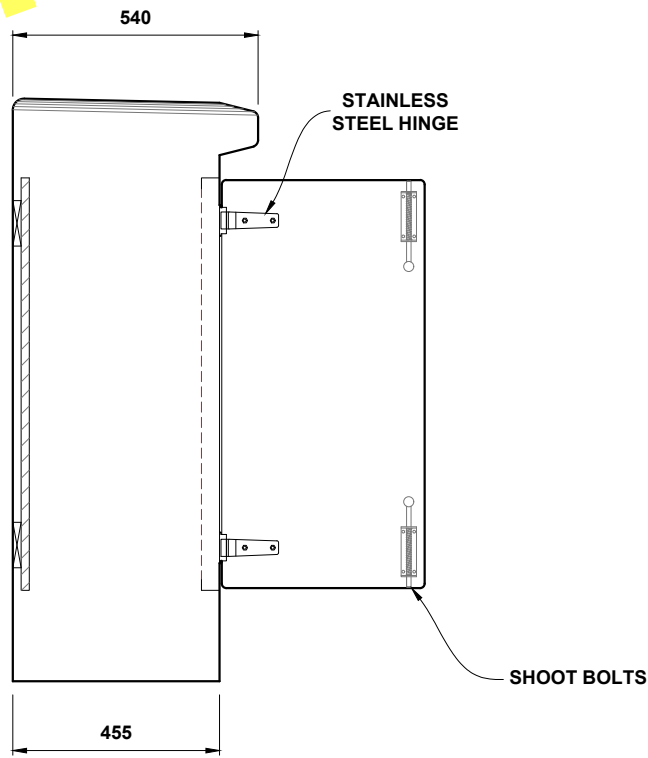
Elevation (C) (l/h side) Door Open
