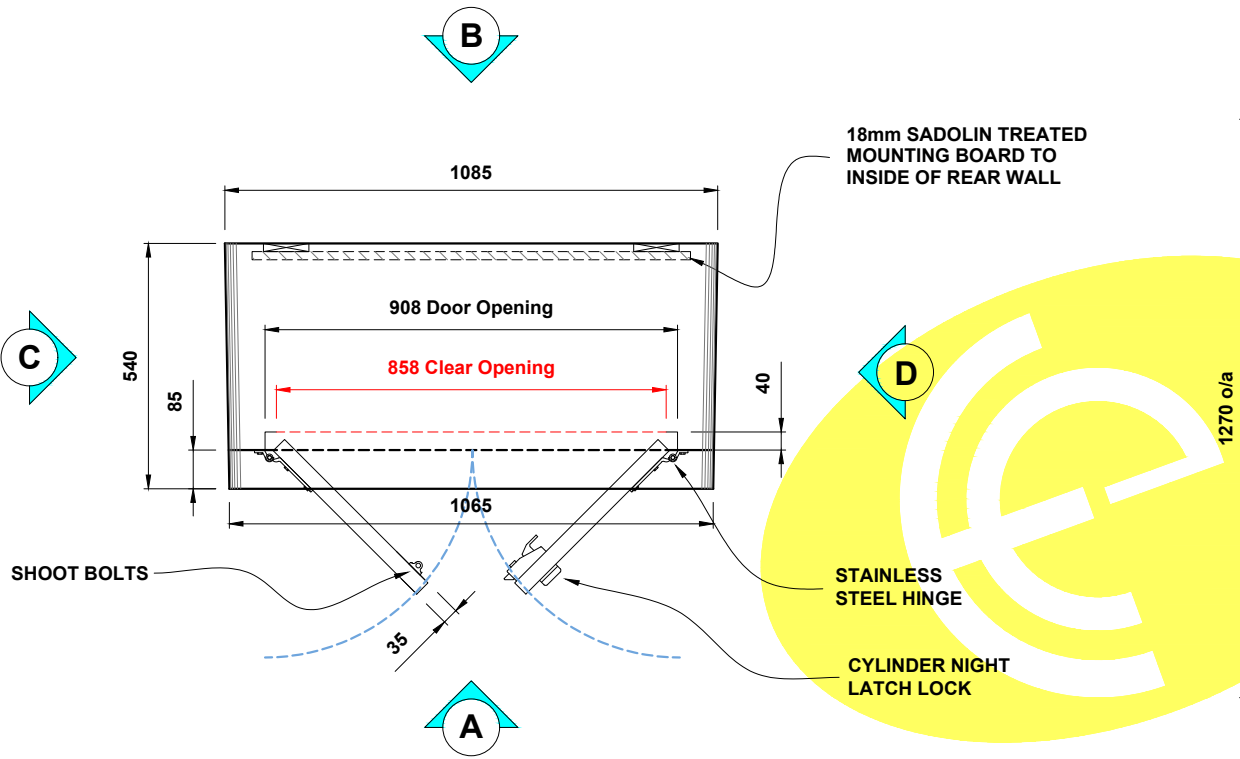
Plan View Elevation - Roadside Range Type O
