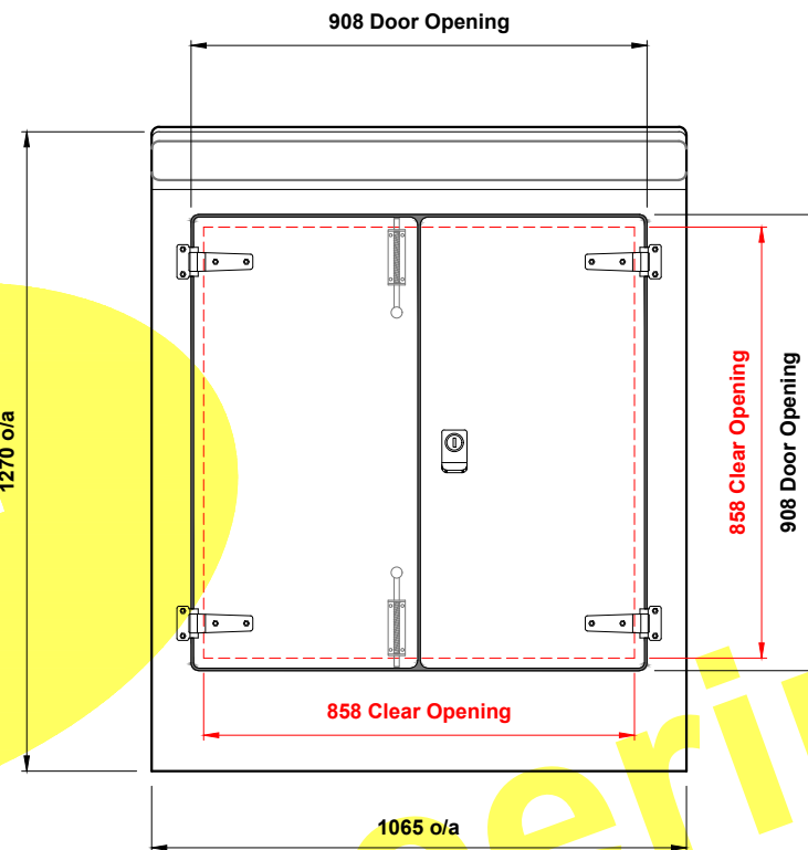
Elevation (A) (front)
