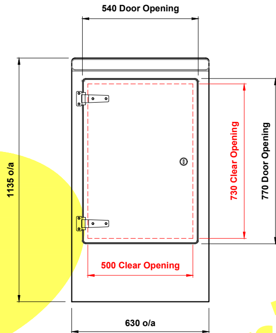
Elevation (A) (front)
