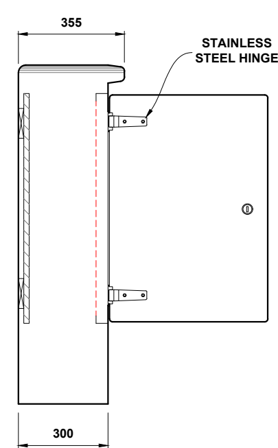
Elevation (C) (l/h side) Door Open
