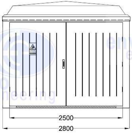
External Elevation Wall 1
